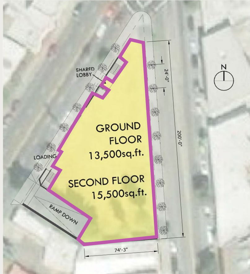
GROUND LEVEL SITE PLAN 1/32" = 1'0"
